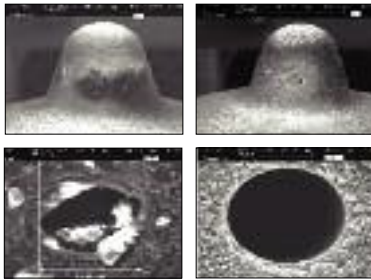
Fuel injector holes show the remarkable difference using basefuel and fuel treated with POWERGUARD™.
